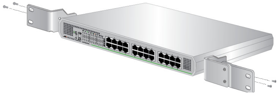
Figure 28. Attaching the Brackets to the Switch
