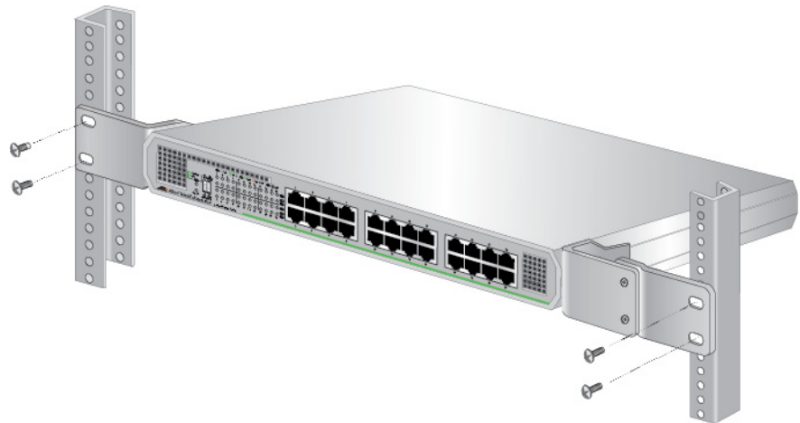
Figure 29. Attaching the Switch to an Equipment Rack
