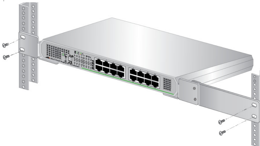
Figure 26. Attaching the Switch to an Equipment Rack
