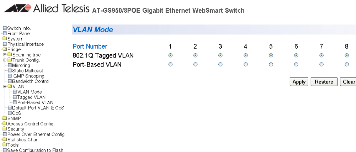
Figure 15. VLAN Mode Page
