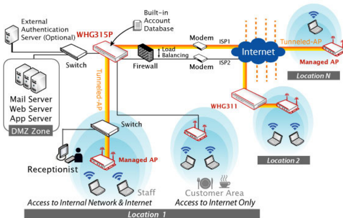
Fig.1. WHG315P in a Business Headquarter
