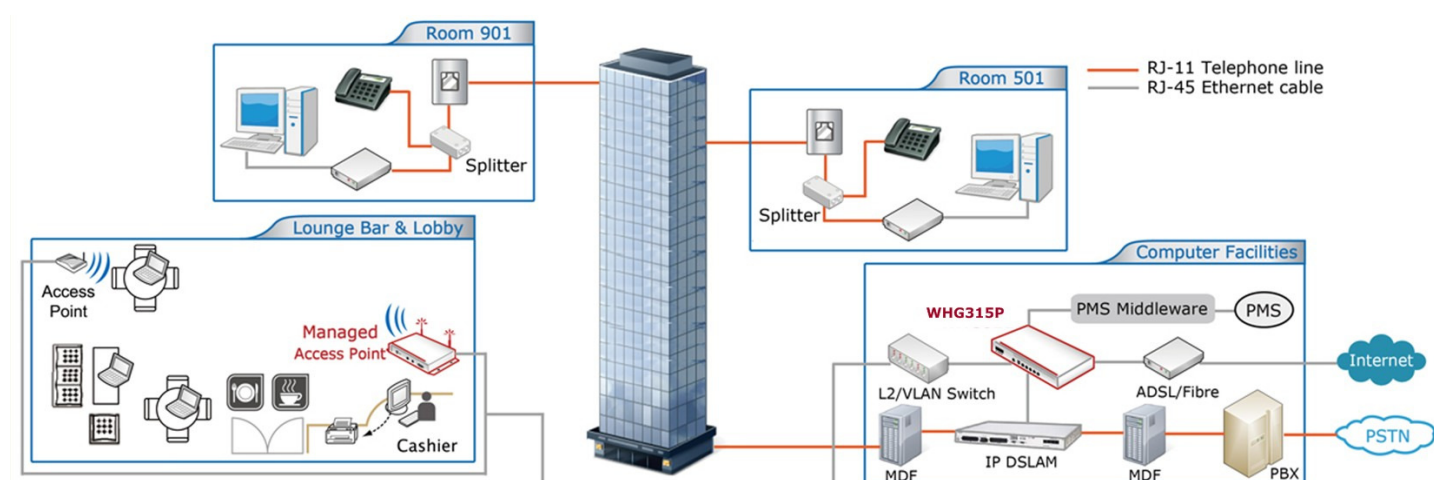
Fig.2. WHG315P in a Hotel - Capable of integrating with DSLAM and PMS
