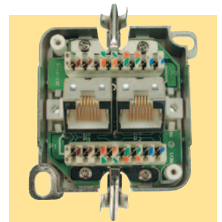
SX8-5E-STP-WH
